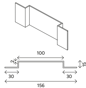
Hutprofil 30/15/100/15/30-2mm in Längen á 6000 mm
